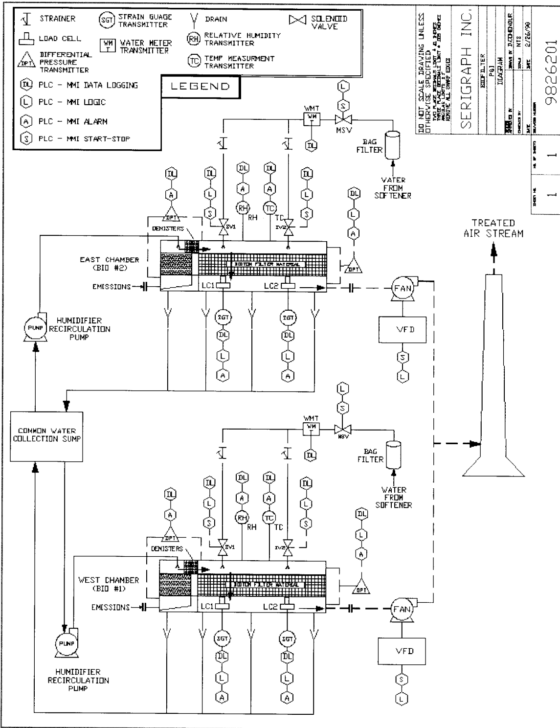
Figure 5. PID Layout of the Biofilter
